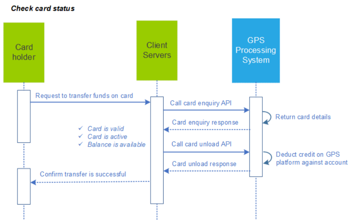
Figure 4: Figure: Using the Card Enquiry web service
