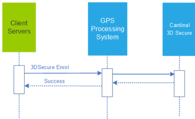
Figure 6: Figure: Using the 3D Secure cardholder enrolment web service
