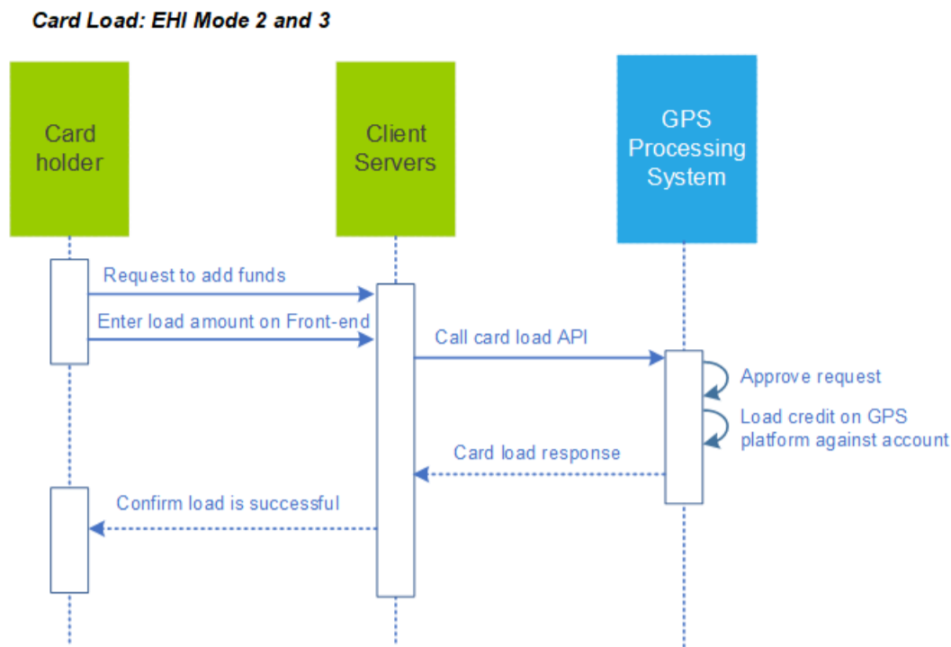
Figure 3: Figure: Using the Card Load web service
