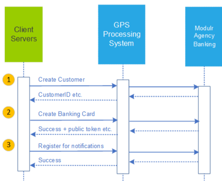
Figure 7: Figure: Using the Modulr Agency Banking Service
