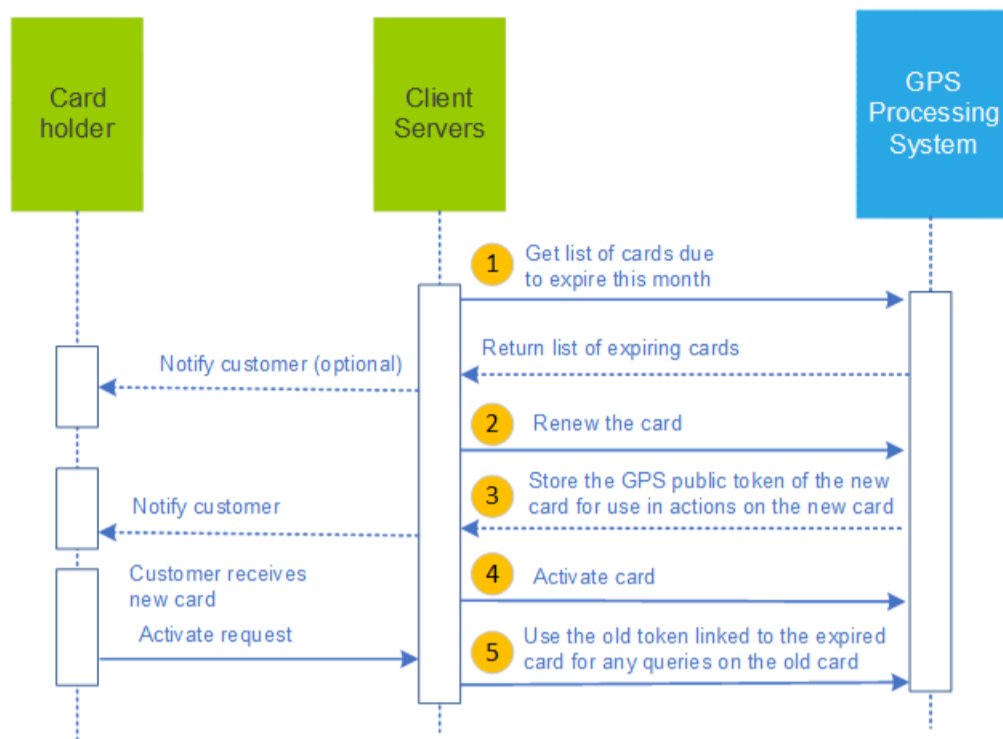
Figure 5: Renewing Expiring Cards
