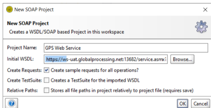
Figure 8: Figure: Starting a new SOAP project and importing the WSDL
