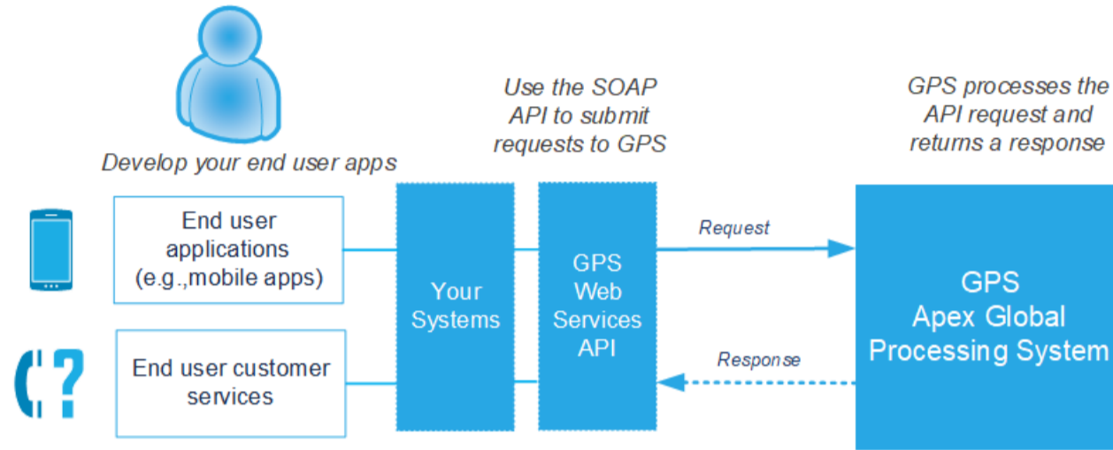
Figure 1: Figure: API Architecture Overview
