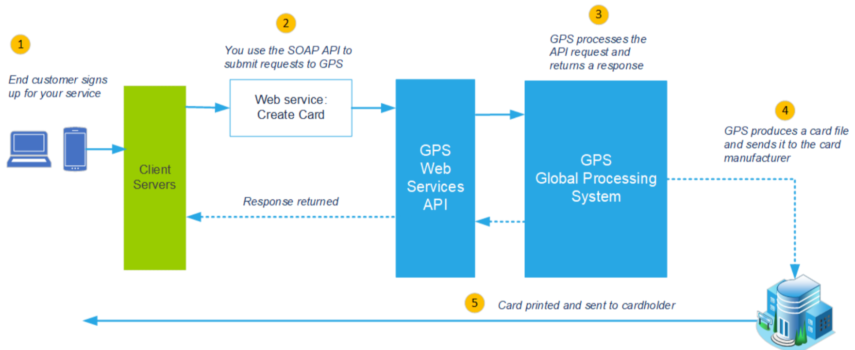
Figure 2: Figure: Using the Card Create web service
